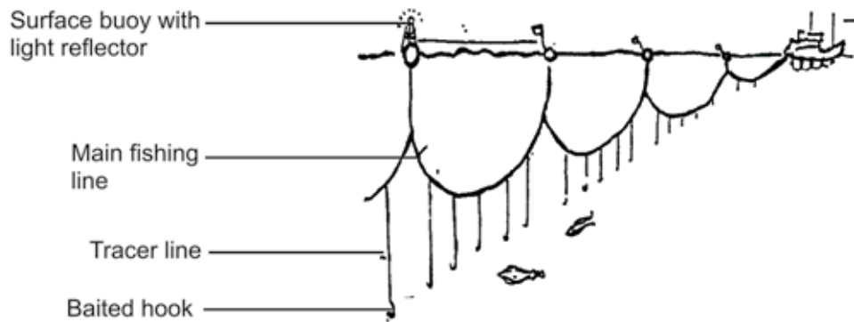
FIGURE 3.5.—Schematic illustration of pelagic longline fishing activity, showing fishing gear deployed in water column ~ 40 m depth (source: D. Japp).
