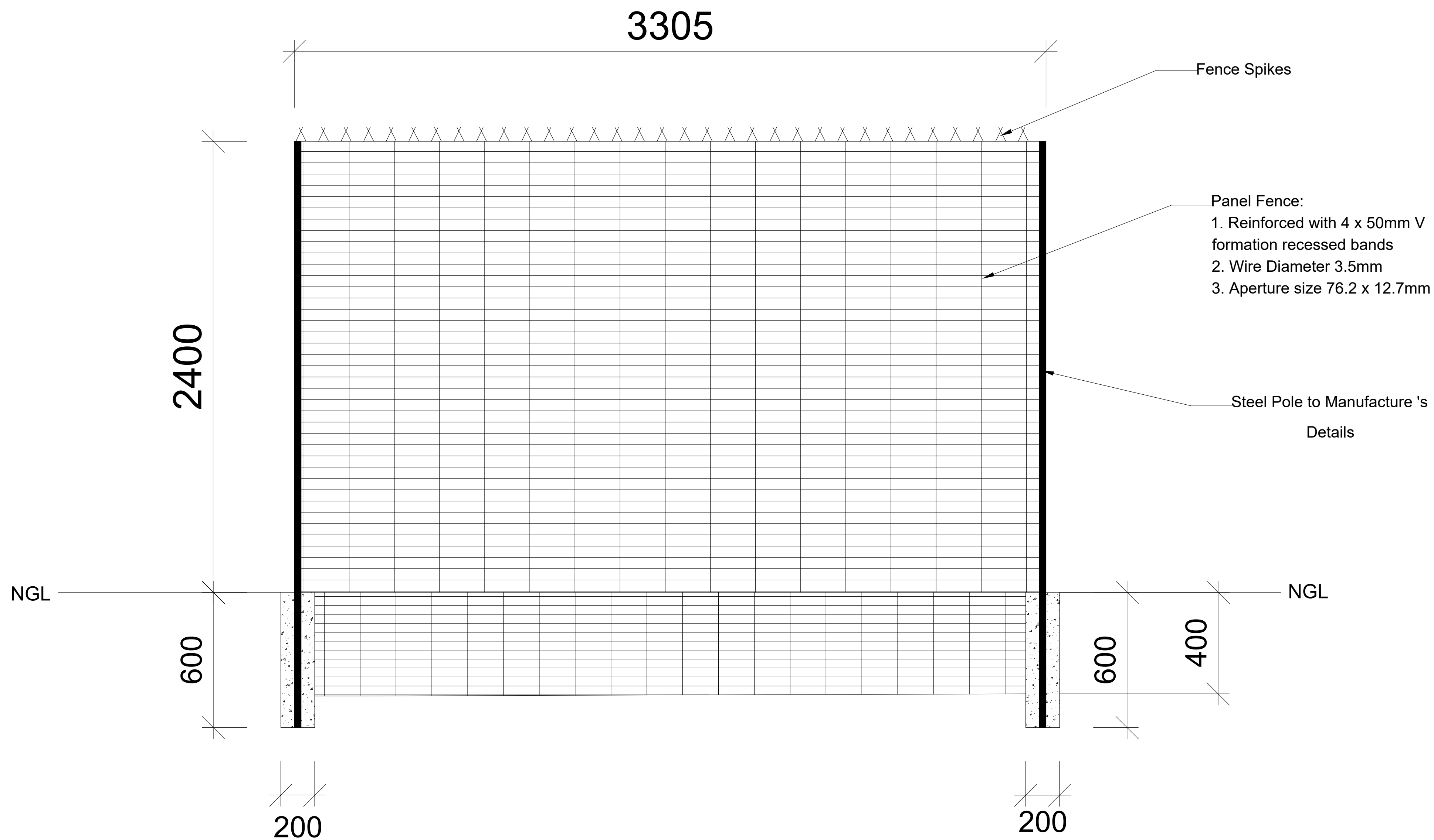
FRONT VIEW HIGH DENSITY FENCE (DETAILS B)
