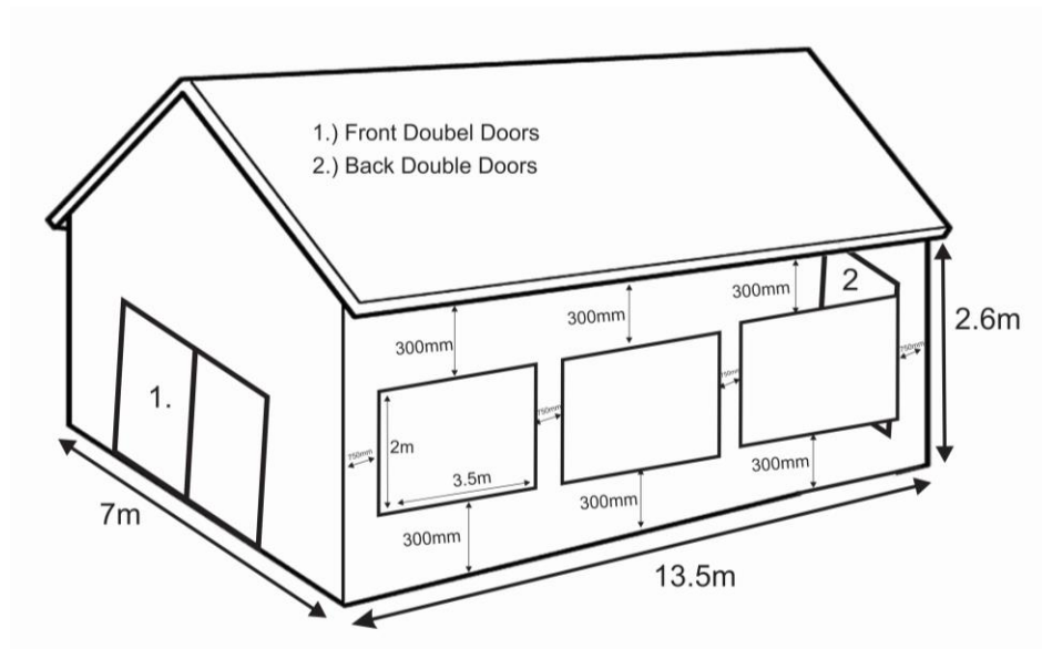
Image 1 : Typical potting shed structure
