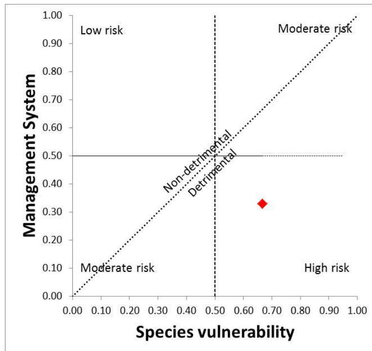
Figure 2. The risk of trading in Encephalartos middelburgensis as represented by the relationship between species vulnerability (biology and status) (0 = low vulnerability; 1 = high vulnerability) and the management system to which the species is subjected (management, control, monitoring, incentives and protection) (0 = weak management system; 1 = strong management system). The figure shows that the species is at high risk and trade is detrimental.
