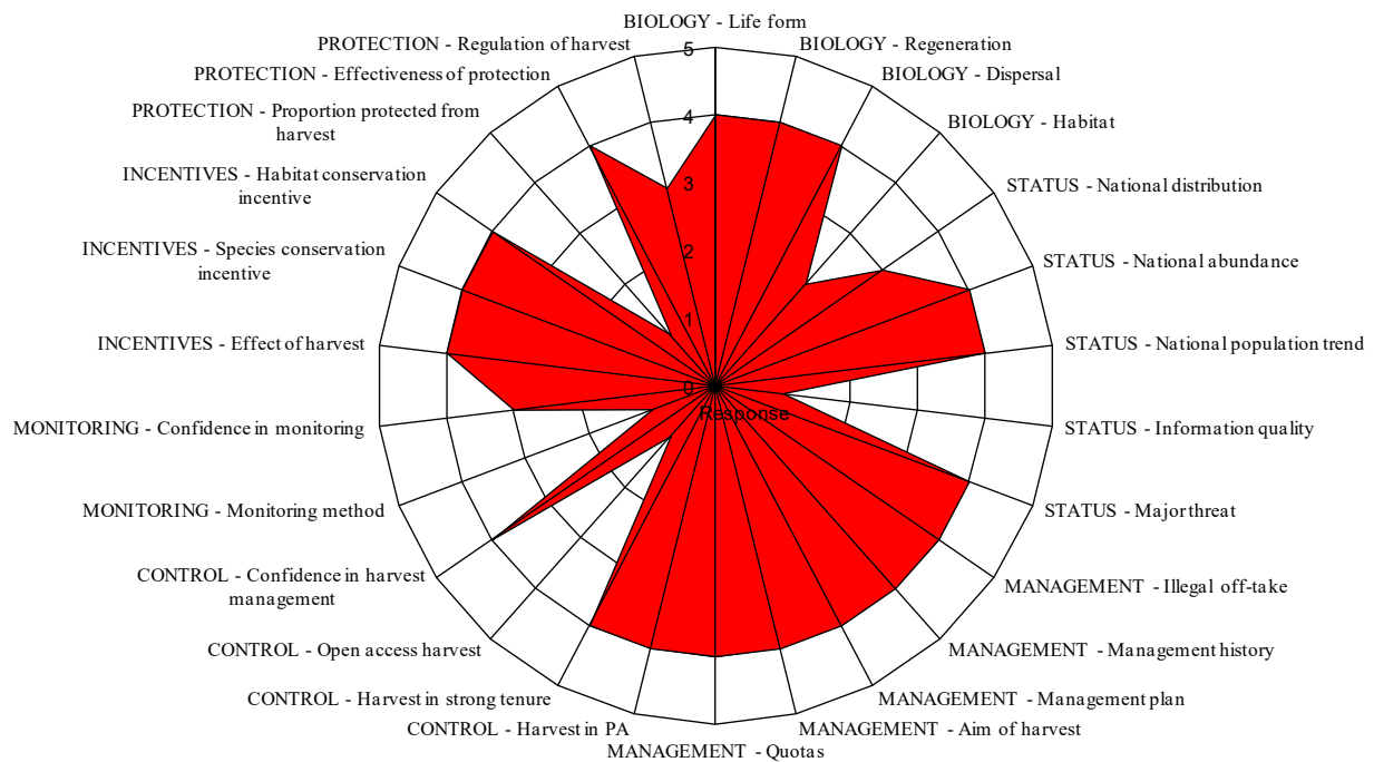
Figure 1. Radar chart summarizing the non-detriment finding assessment undertaken for Encephalartos middelburgensis in accordance with the CITES NDF checklist. Explanations of scores given are detailed in Table 1. Higher scores are indicative of higher risks to the species. The extensive shaded area in the radar chart demonstrates an overall high risk to the species.
